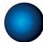
Neutron, n
