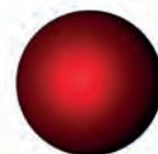
Proton, p^+
